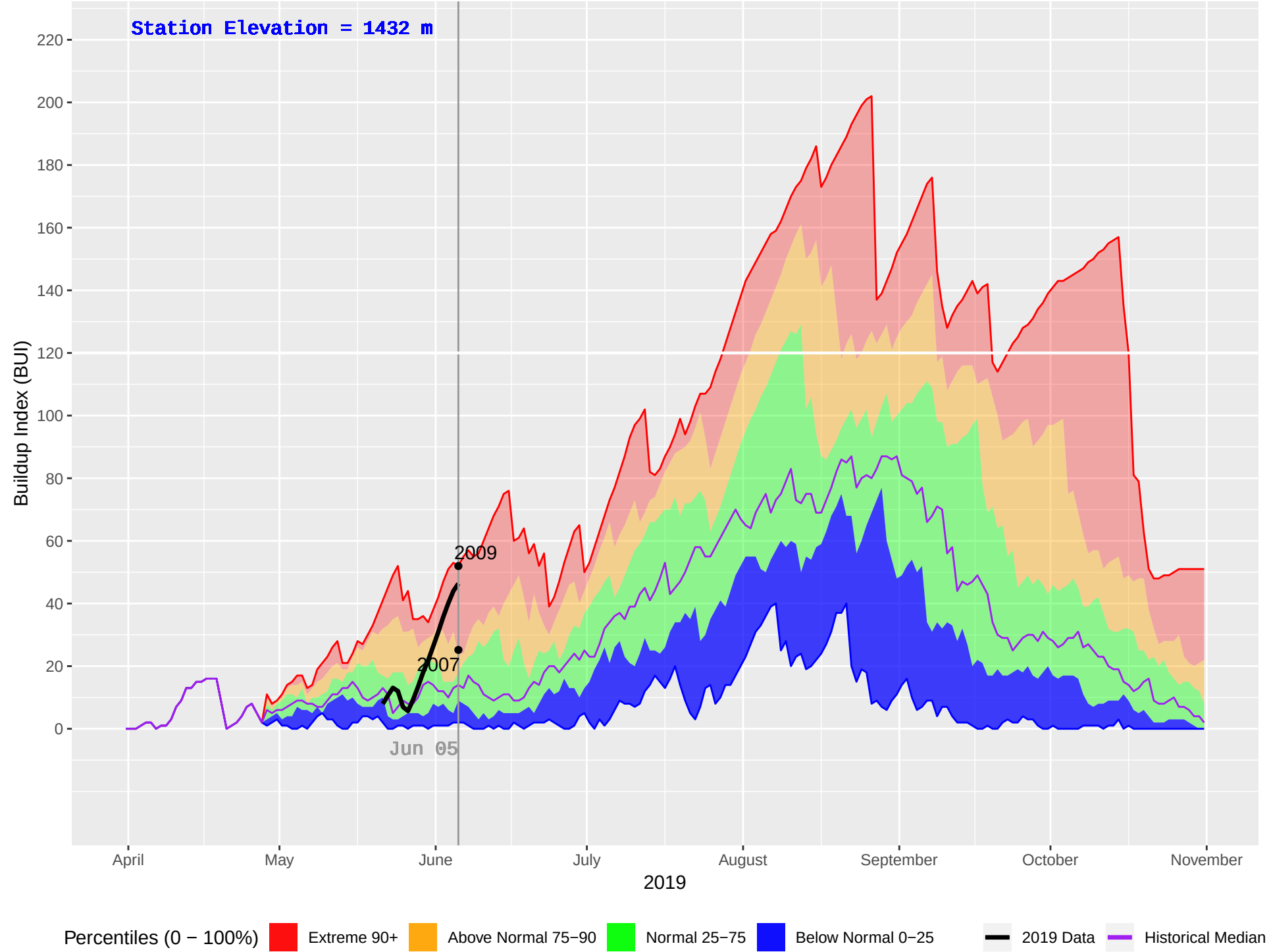
OCTOPUS CREEK (396) : Historical (2000–2018), Current (2019) Daily Buildup Index (BUI)
