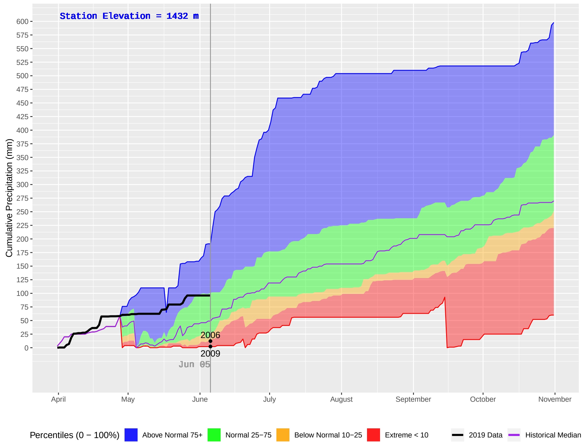
OCTOPUS CREEK (396) : Historical (2000–2018), Current (2019) Daily Cumulative Precipitation
