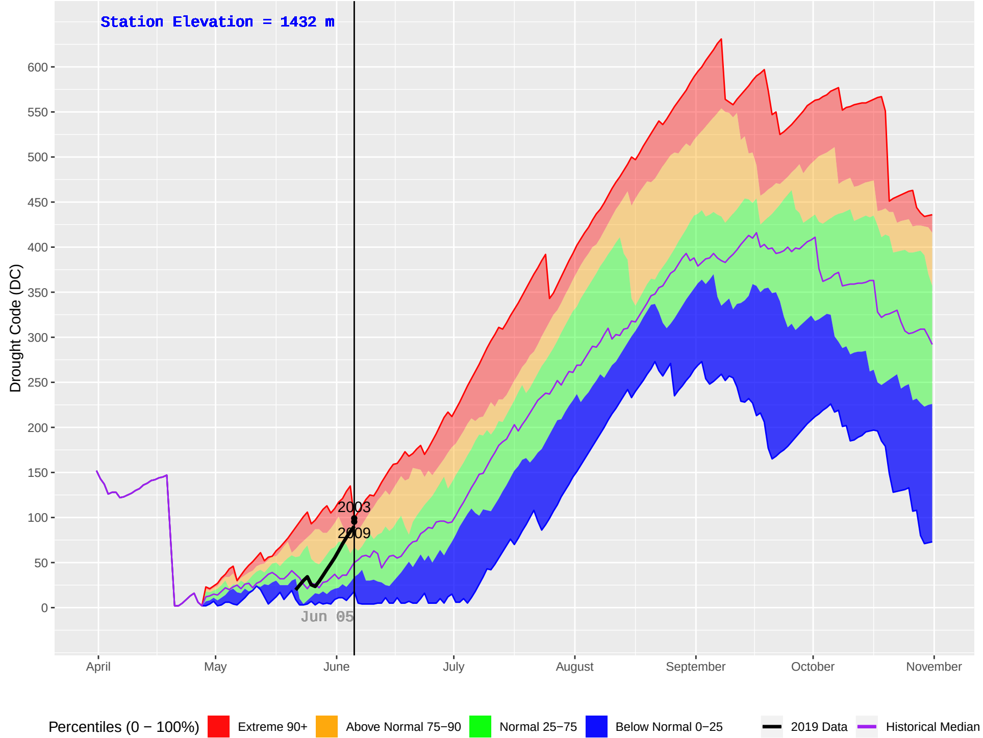
OCTOPUS CREEK (396) : Historical (2000–2018) and Current (2019) Daily Drought Code (DC)
