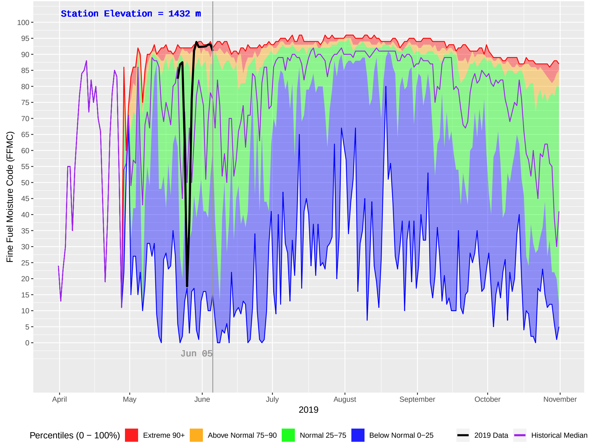
OCTOPUS CREEK (396) : Historical (2000–2018) and Current (2019) Daily Fine Fuel Moisture Code (FFMC)
