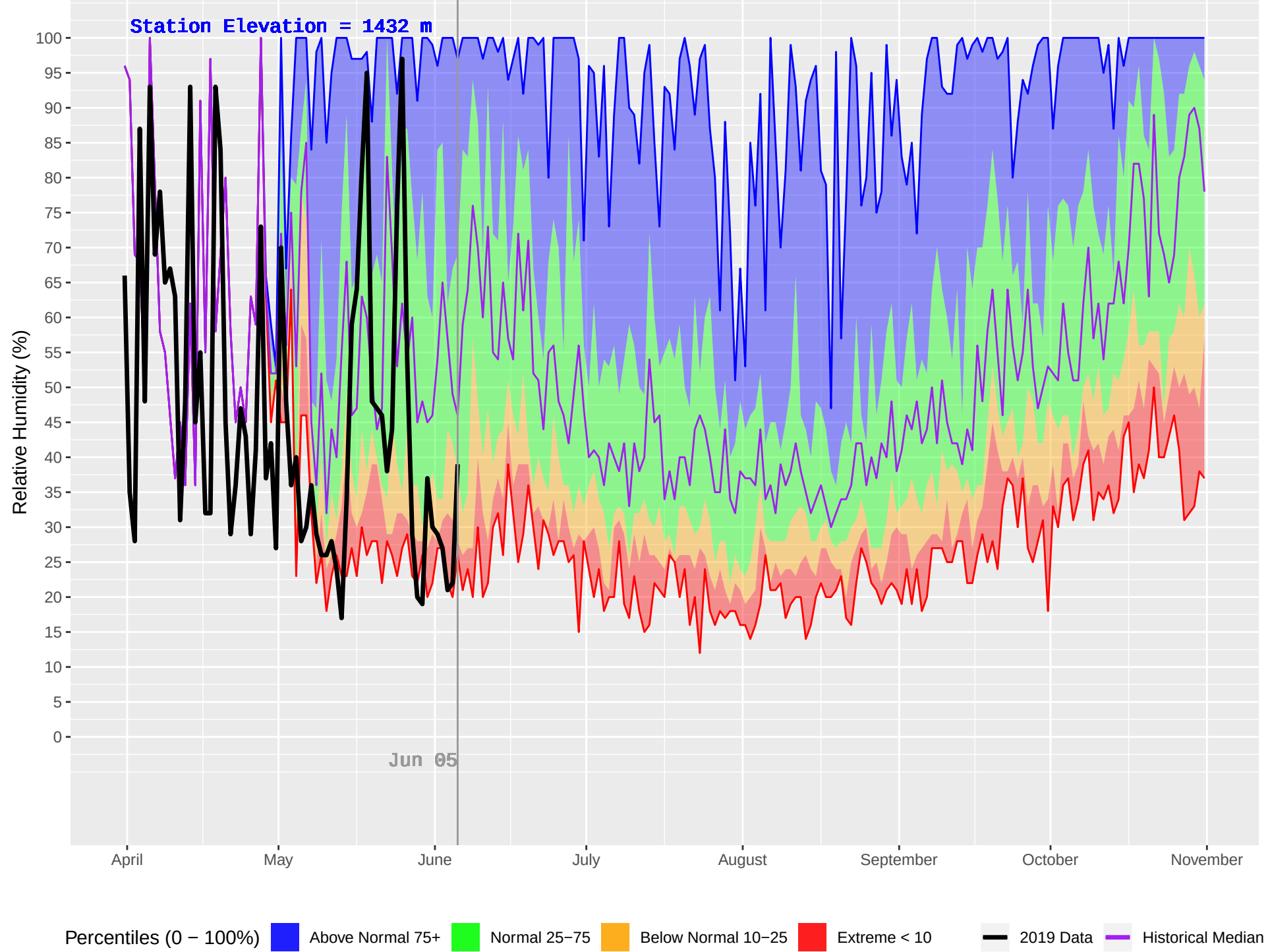
OCTOPUS CREEK (396) : Historical (2000–2018) and Current (2019) Daily Relative Humidity
