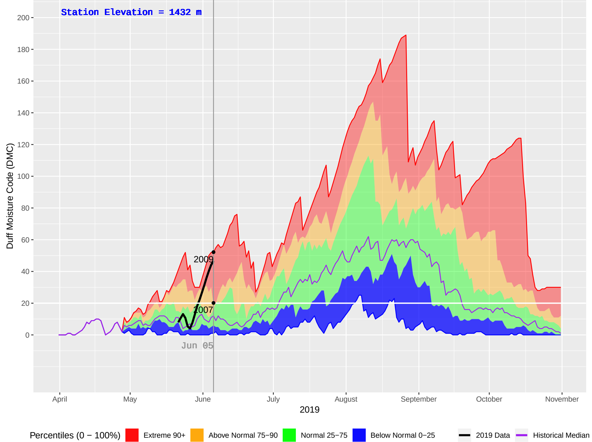
OCTOPUS CREEK (396) : Historical (2000–2018), Current (2019) Daily Duff Moisture Code (DMC)
